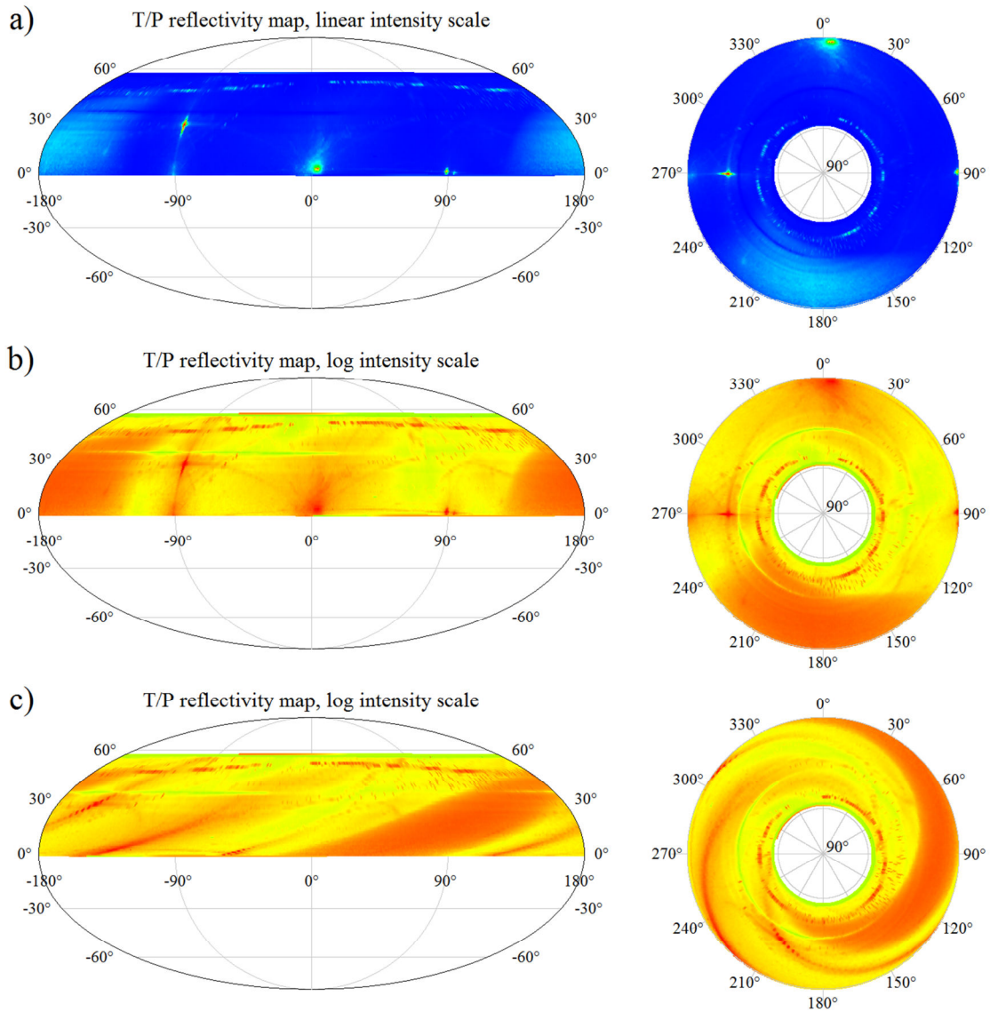
Fig. 4. TOPEX reflectivity map presented in the Mollweide (the prime meridian indicates front of the satellite body) and polar (only northern hemisphere) projections. A) reflection intensity in the linear scale, b) logarithmic scale, c) the pattern distortion caused by 100 ms increase in the spin period.
