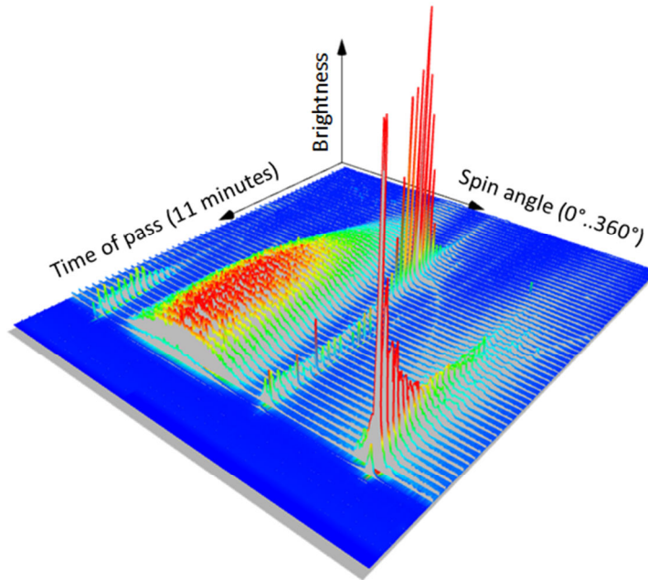
Fig. 3. The phase-folded high-rate light curve of TOPEX/Poseidon measured by Graz system.
