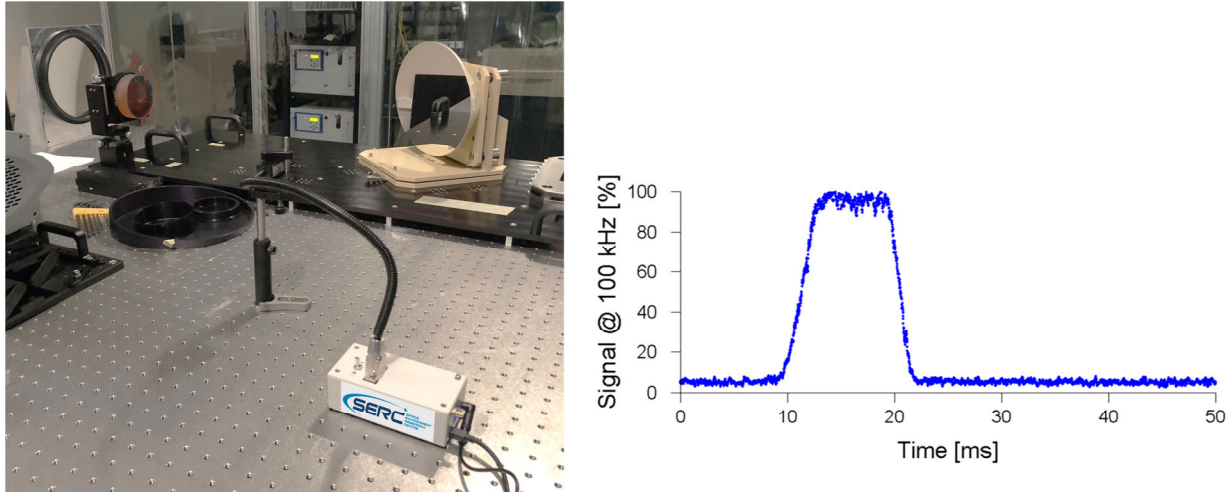
Fig. 5. Left: the high-rate photometric detector during the laboratory tests (Mount Stromlo). Right: Ajisai solar flash measured by the SERC high-rate detector at 100 kHz sampling rate.
