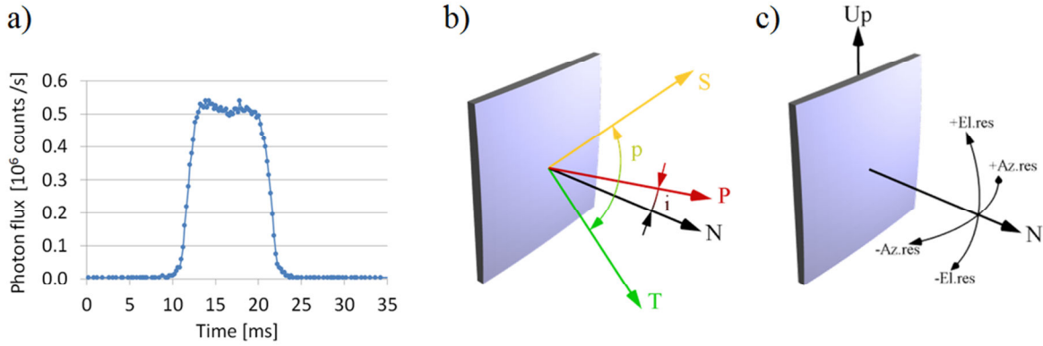
Fig. 1. A) solar flash from a single Ajisai mirror measured by Graz photometric system. B) the vector/angle system used in the analysis of the specular reflections: Sun S , telescope T , surface normal N , phase vector P , phase angle p , inclination angle i . C) Deviation of the phase vector P from the normal N can be defined by azimuth and elevation residual angles; the Up direction points towards the top of the satellite body.
