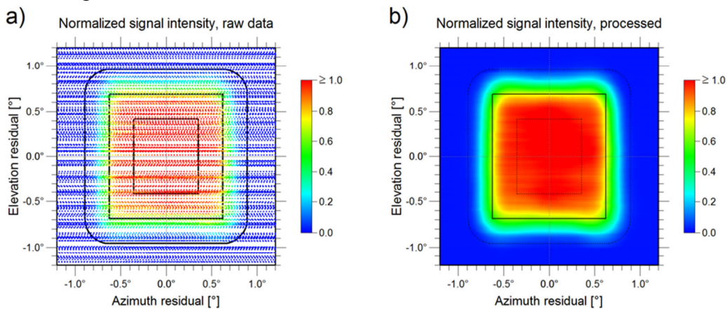
Fig. 2. An example reflectivity profile of a single mirror panel (approx. size of 20 x 20 cm) of Ajisai determined by HDP. A) normalized photometric observation at the angular coordinates of the corresponding phase vector. B) the post-processed reflectivity map of the panel. The inner rectangular frame represents the maximum reflectivity area defined by a slight convex curvature of the panel; the middle frame is the angular size of the mirror and the outer frame limits the reflectivity area of the mirror.
