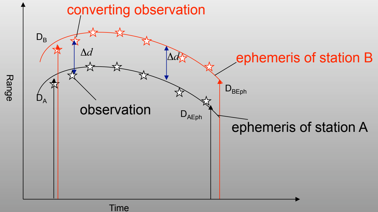
Figure 1. The conditional image of a differential method
