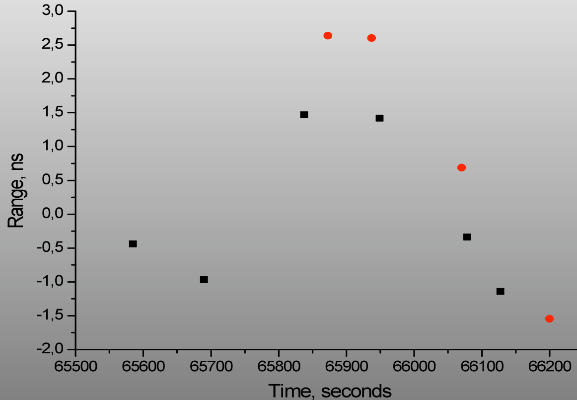
Figure 4. Difference between observations and ephemeris of station Simeiz (black) and difference between transformation observations of station Katzively and ephemeris of station Simeiz (red), satellite LAGEOS 1 for 31.03.2004
