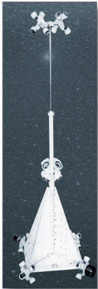
Figure 3-2. A distributed array of cornercubes on the Reflector Satellite is used to study spacecraft dynamics.
